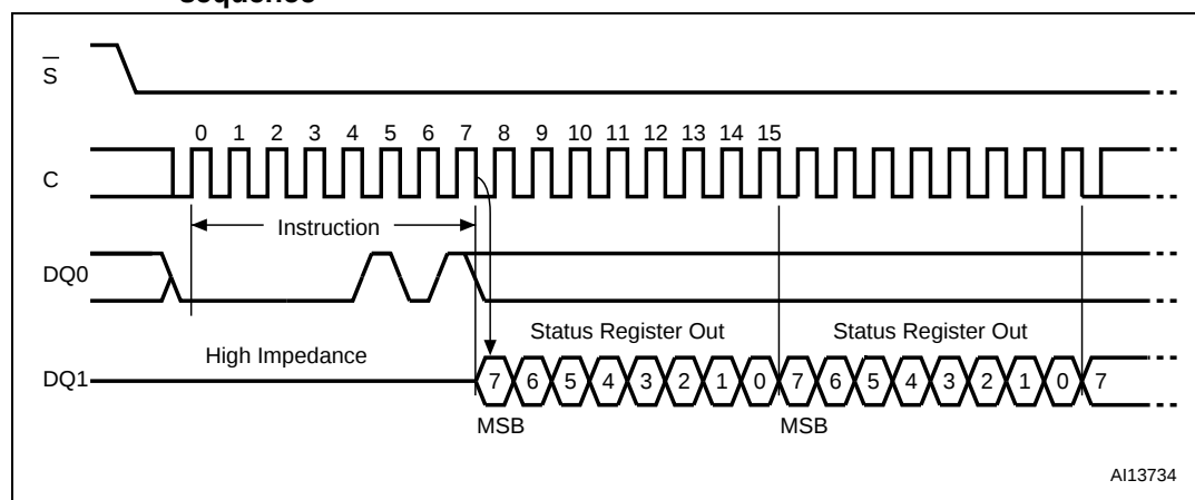
Figure 12. Read Status Register (RDSR) instruction sequence and data-out sequence
