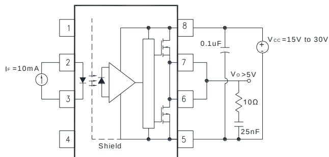
Figure 18 : I_{FLH} Test Circuit
