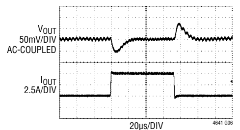
1V Transient Response, 38V IN
