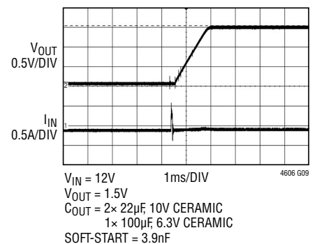
-55°C, Start-Up, I OUT = 0A
