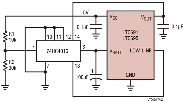
Capacitor Back-Up with 74HC4016 Switch
