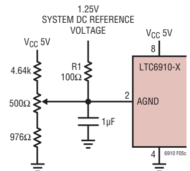
Figure 5c. Offset Nulling (Single Supply, External Reference)
