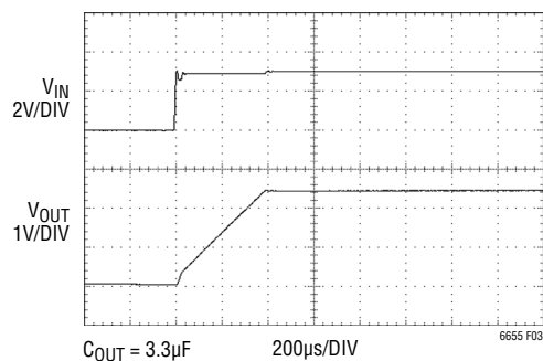
Figure 3. Start-Up Response
