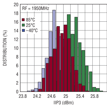
IIP3 Distribution
