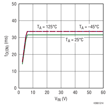
GATE Turn-On Delay Time vs V_{IN}
