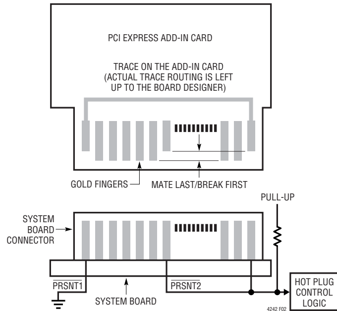
Figure 2. Plug-In Card Insertion/Removal
