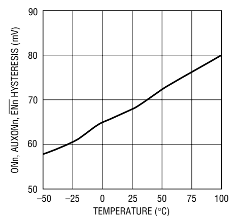
ONn , AUXONn , \overline{ENn} Hysteresis vs Temperature
