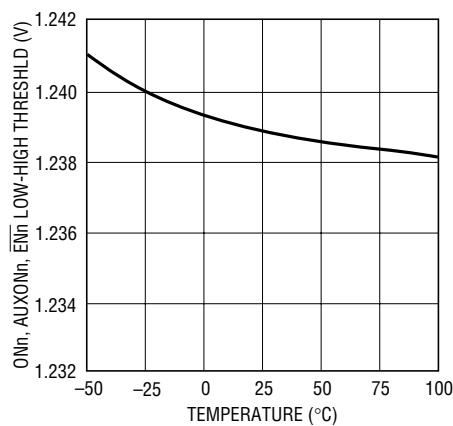
ONn , AUXONn , \overline{ENn} Low-to-High Threshold vs Temperature
