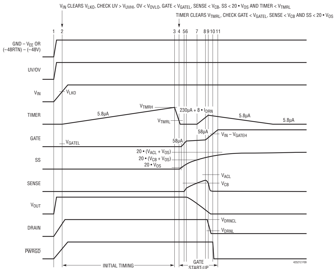
Figure 9. System Power-Up Timing (All Waveforms Are Referenced to V_{FF} )
