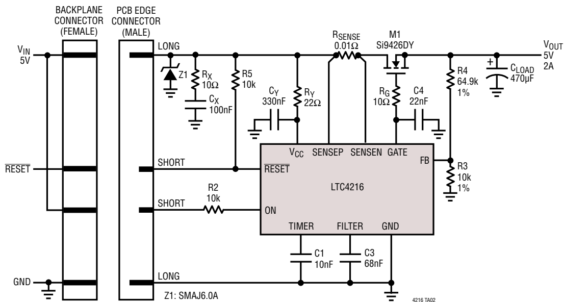
LTC4216CMS with Gate Capacitor for Slew Rate Control
