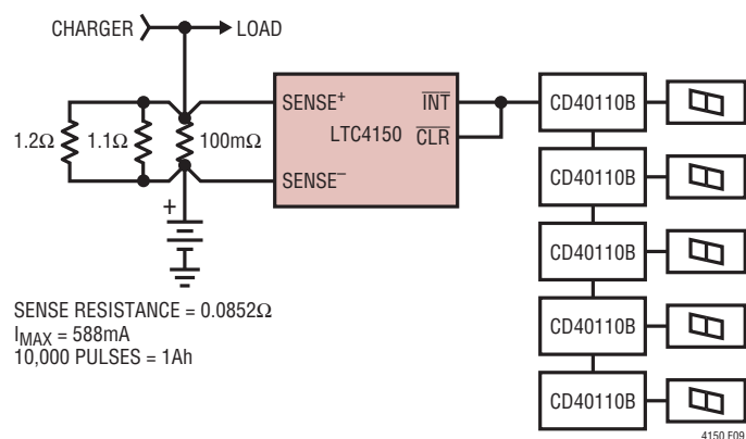
Figure 9. Ampere-Hour Gauge
