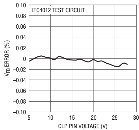
V_{\text{FB}} Line Regulation
