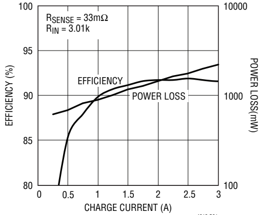
Efficiency at \text{DCIN} = 20\text{V} , \text{BAT} = 8\text{V}
