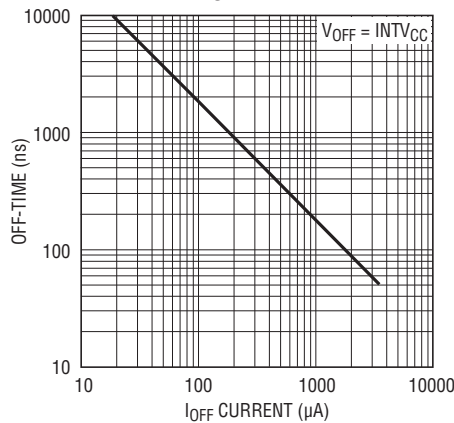
Off-Time vs I_{OFF} Current
