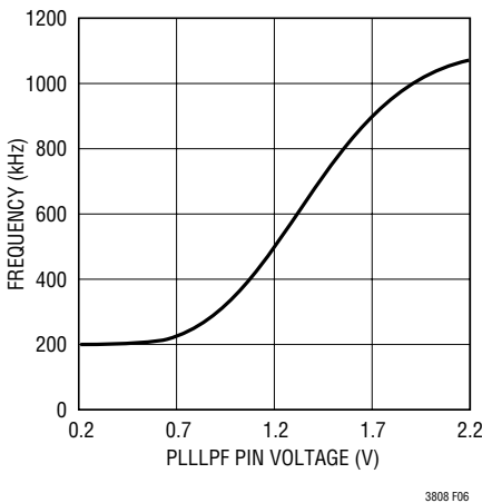
Figure 6. Relationship Between Oscillator Frequency and Voltage at the PLLPF Pin When Synchronizing to an External Clock
