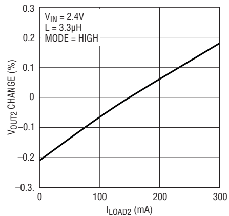
V_{OUT2} = 3.3\text{V} Load Regulation
