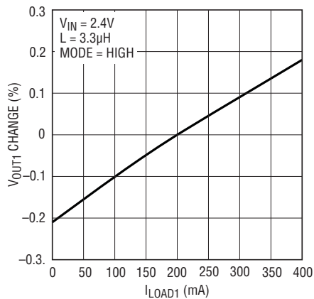
V_{OUT1} = 5\text{V} Load Regulation
