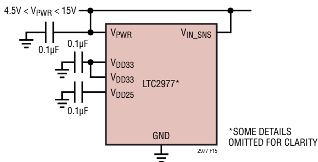
Figure 15. Powering LTC2977 Directly from an Intermediate Bus
