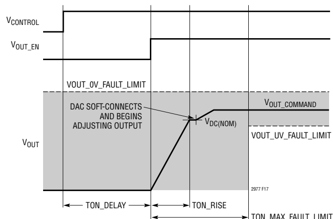
Figure 17. Typical On Sequence Using Control Pin
