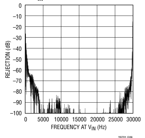
ADC Rejection vs Frequency at V_{IN}
