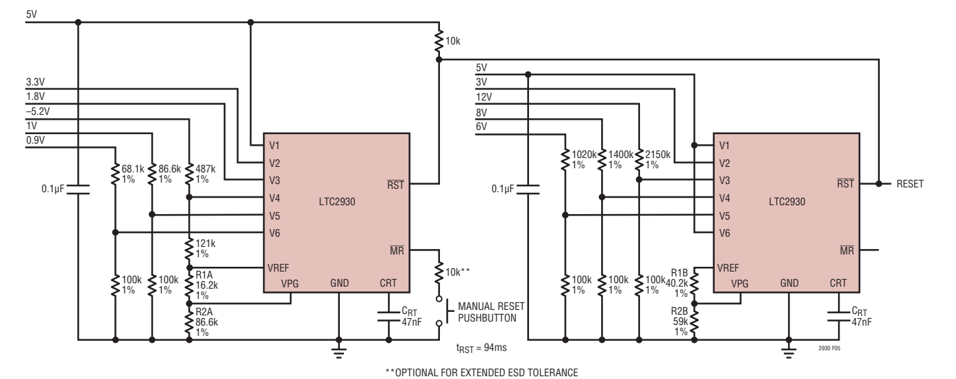
Figure 5. OR-ed System Reset
