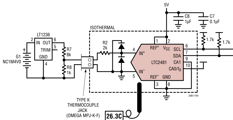
Figure 44. Calibration Setup
