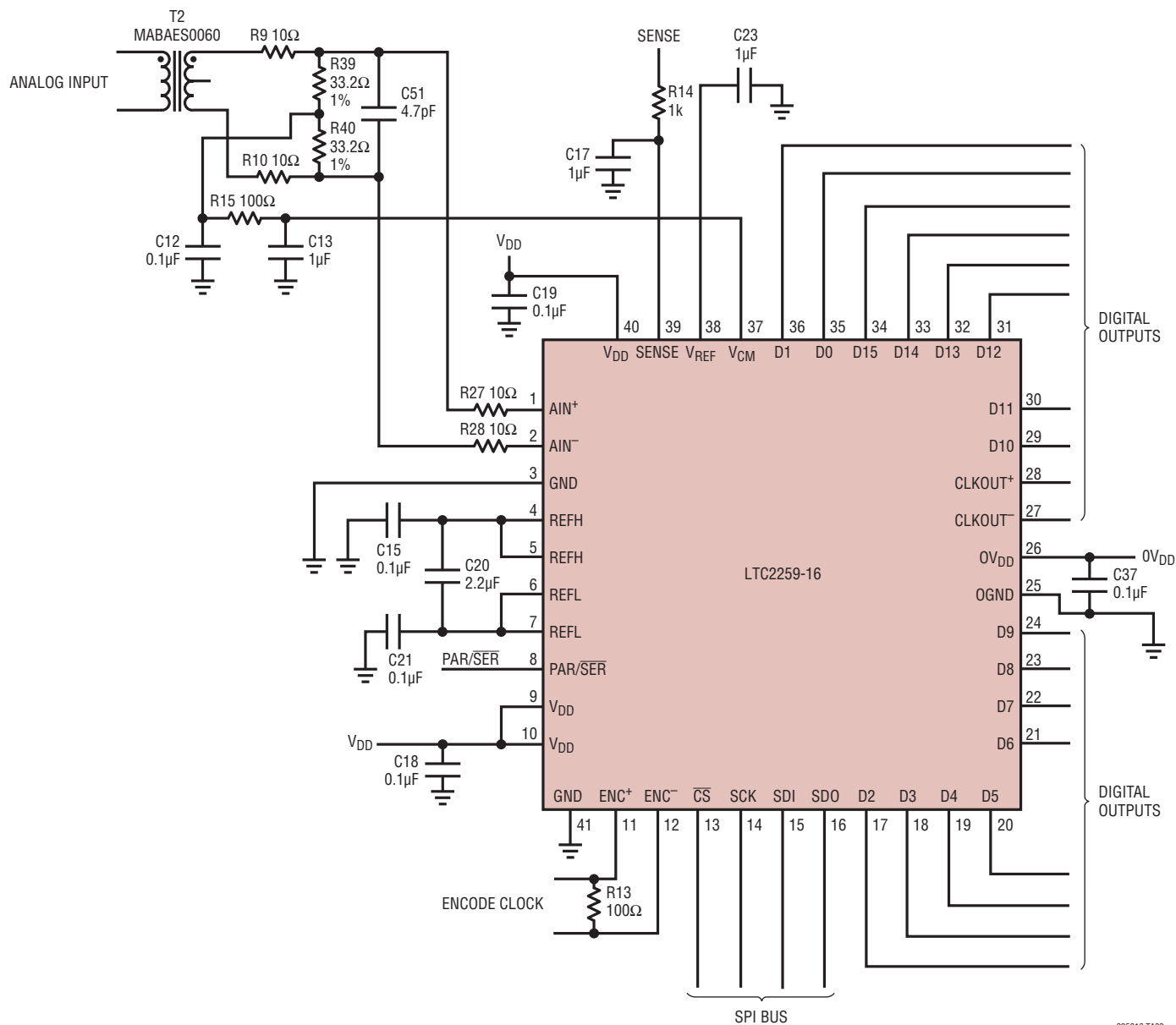
LTC2259-16 Schematic
