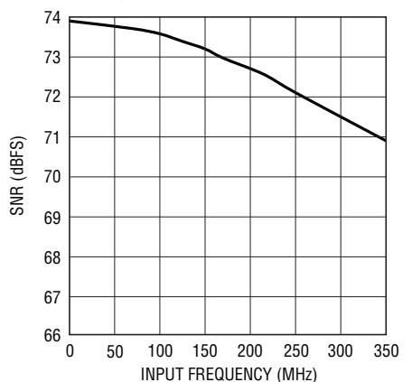
LTC2258-14: SNR vs Input Frequency, -1\text{dB} , 2\text{V} Range, 65\text{Msps}
