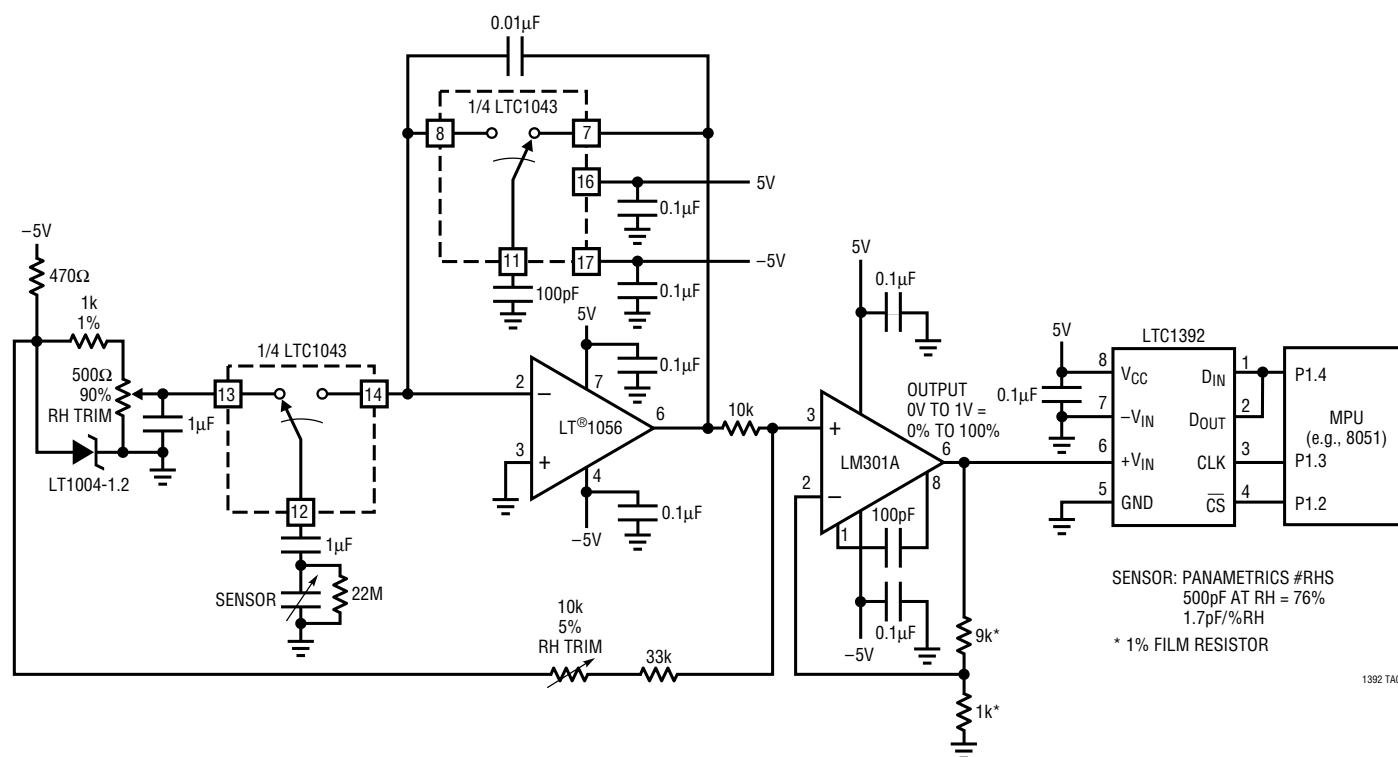
System Monitor for Relative Humidity, Supply Voltage and Ambient Temperature
