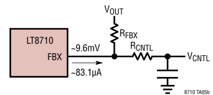
Schematic and Equations for Calculating V_{OUT}
