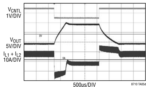
Transient Response with Stepping V_{\text{CNTL}} from 0V to -1V to 0V with 2\Omega Output Load
