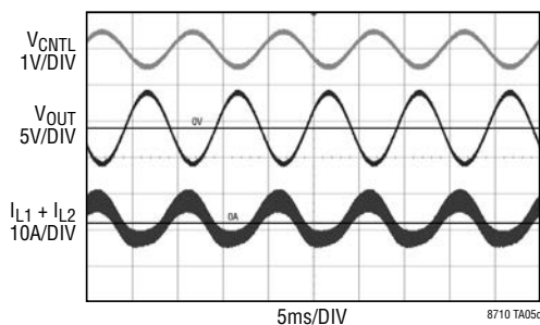
V OUT Cleanly Transitions Through 0V with a 1V, 100Hz Sine Wave CNTL Signal (R LOAD = 2Ω)
