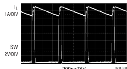
Switching Waveforms
