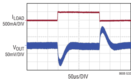
Transient Response
