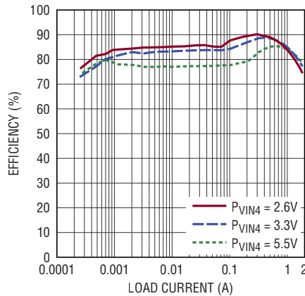
LV Channel Efficiency vs Load V_{OUT4} = 1.2\text{V} , F_{SW} = 2\text{MHz}
