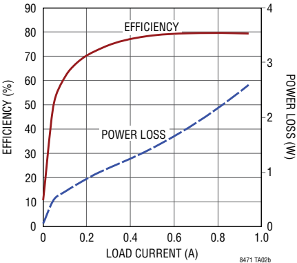
Efficiency and Power Loss V_{CC} = 12V , with Load Current from V_{OUT2} to V_{OUT1}
