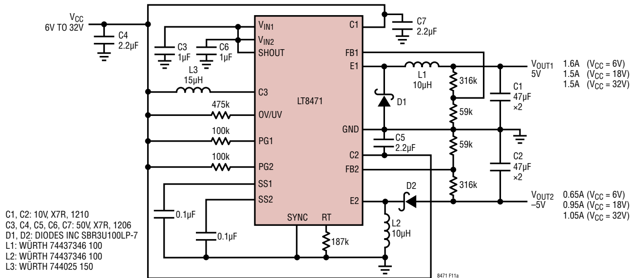
Figure 11a. Wide Input Range Converter with \pm 5V Output Voltages at 450kHz
