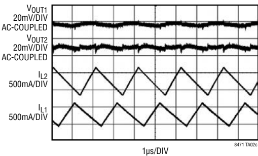
Output Voltage Ripple in CCM, V_{CC} = 10V
