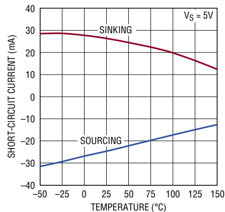
Short-Circuit vs Temperature
