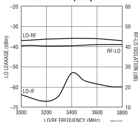
LO Leakage and RF-LO Isolation vs LO and RF Frequency
