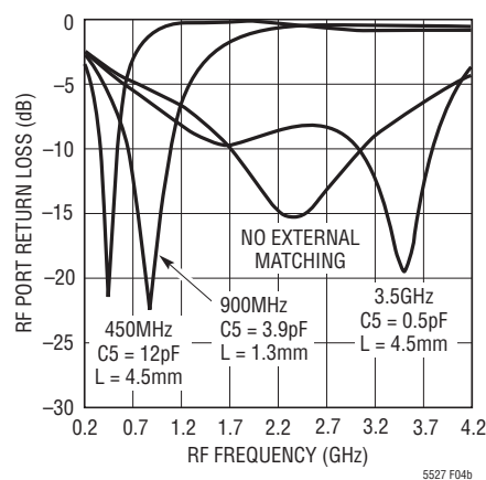
(4b) Series Shunt Matching
