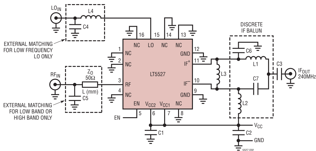
Figure 1. Downmixer Test Schematic—Standard IF Matching (240MHz IF)
