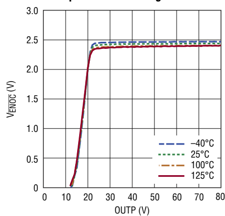
\overline{EN} Open Circuit Voltage
