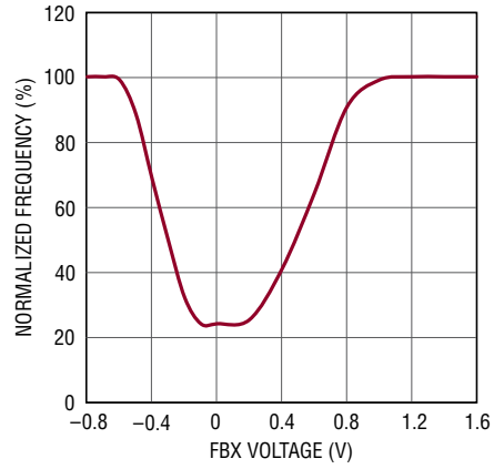
Normalized Switching Frequency vs FBX
