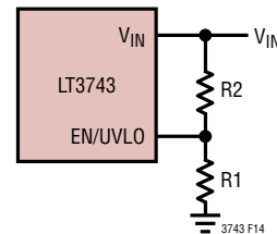
Figure 14. UVLO Configuration
