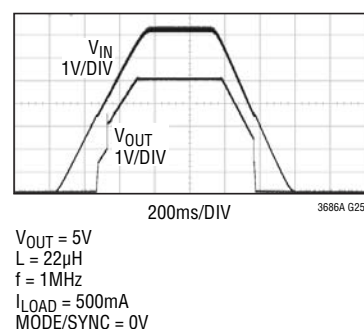
Start-Up Shutdown Waveform I_{LOAD} = 500\text{mA}
