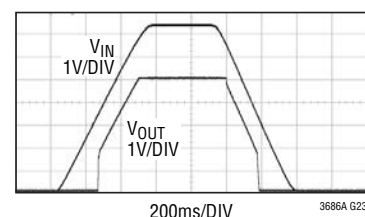
Start-Up Shutdown Waveform I_{LOAD} = 5\text{mA}
