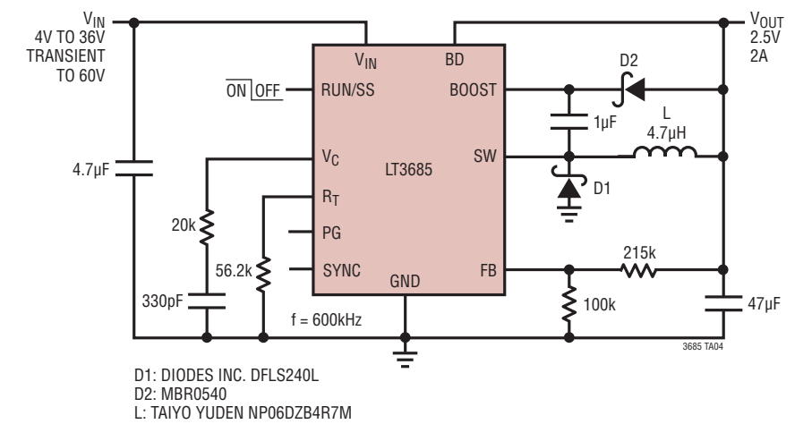
2.5V Step-Down Converter
