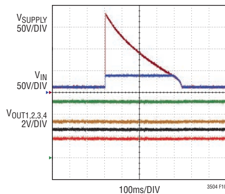
Figure 10. Overvoltage Protection Withstands 180V Surge
