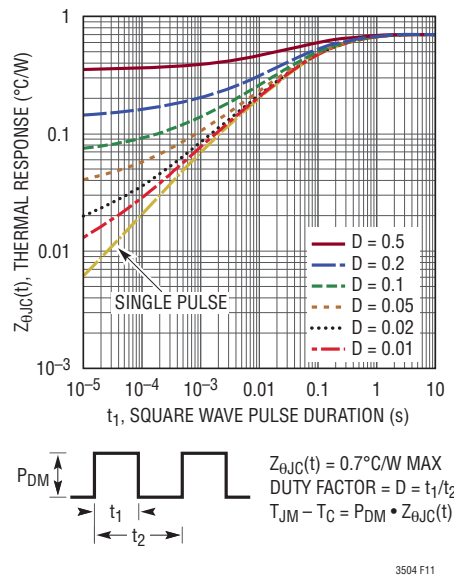
Figure 11. FQB34N20L Transient Thermal Response
