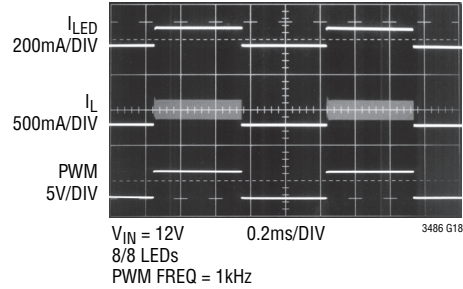
PWM Dimming Wavforms
