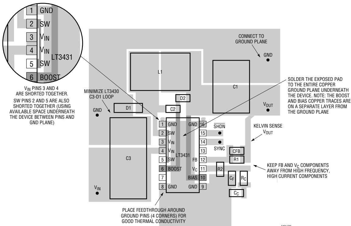
Figure 6. Suggested Layout
