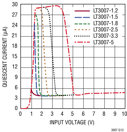
Quiescent Current
