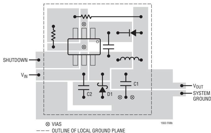
(8b) SOT-23 Package
