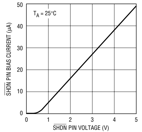
\overline{\text{SHDN}} Pin Current vs V_{\overline{\text{SHDN}}}
