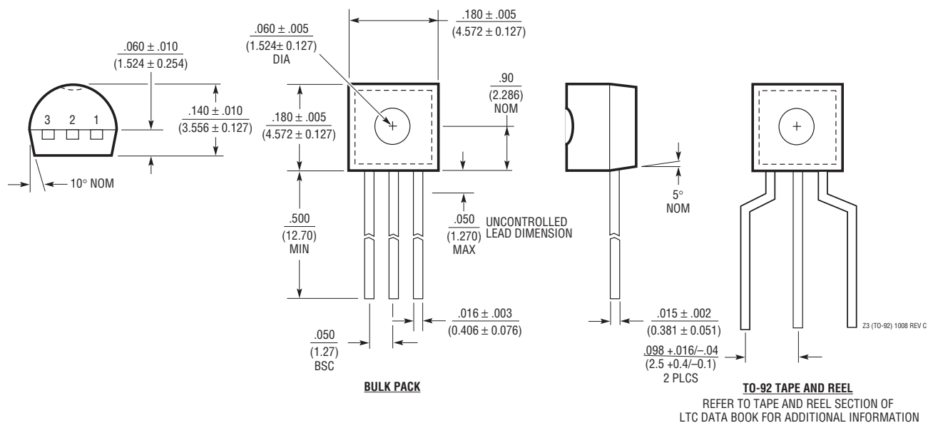
Z Package 3-Lead Plastic TO-92 (Similar to TO-226) (Reference LTC DWG # 05-08-1410 Rev C)
