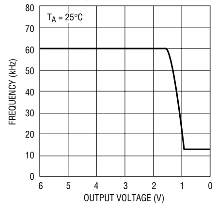
Telecom 5V Supply Short-Circuit Frequency Shift-Down
