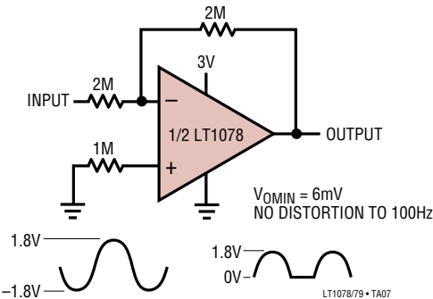
Half-Wave Rectifier
