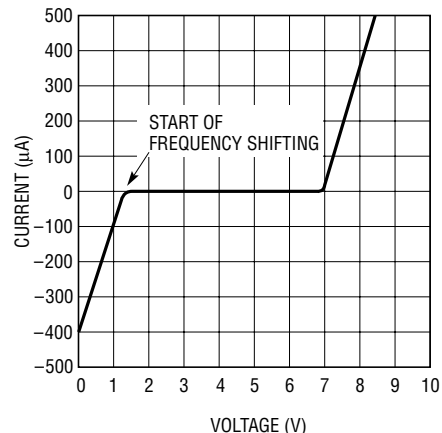
Feedback Pin Characteristics
