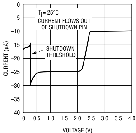
Shutdown Pin Characteristics
