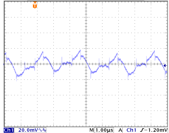
Output Ripple & Noise ( V_{IN} = 12V , I_{OUT} = 20A , C_{OUT} = 10\mu F || 1\mu F , 'scope = 20 MHz BW) Vertical = 20 mV/div., Sweep = 1 \mu S/div.
