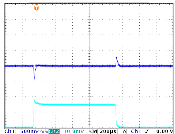
StepLoad Transient Response ( V_{IN} = 12V , 0-15A-0)
