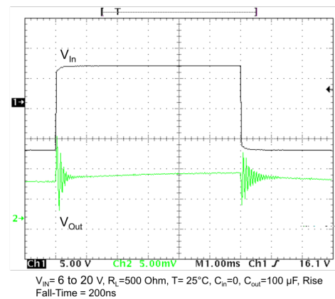
Figure 23. Line transient
