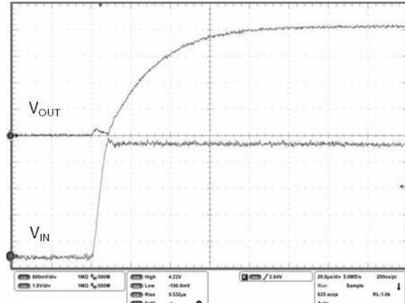
Figure 30. Startup transient
