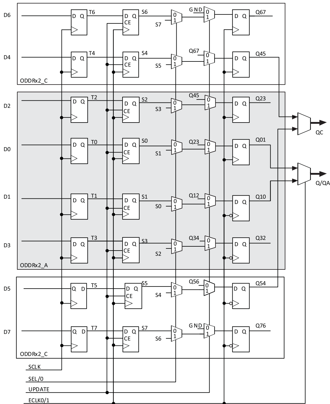
Figure 2.17. Output Gearbox
