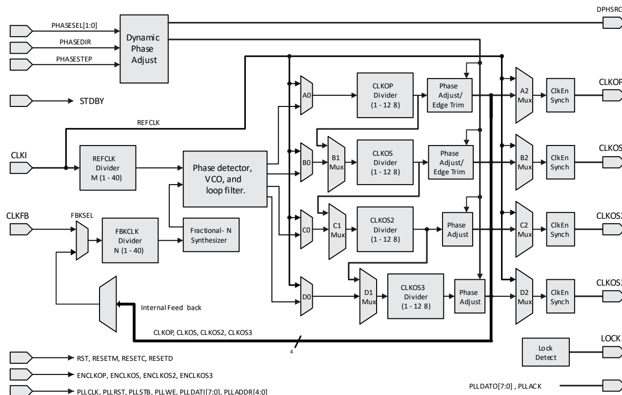
Figure 2.7. PLL Diagram
